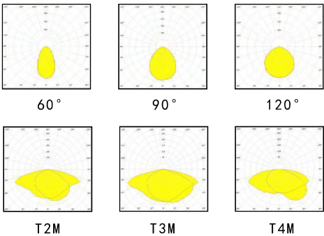
配光曲线/Distribution curve
