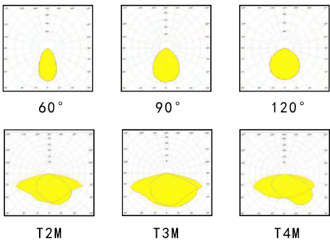
配光曲线/Disrtibution curve
